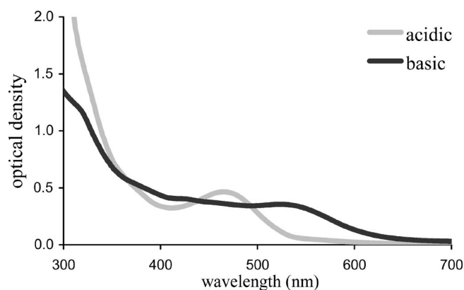
Figure 1. UV/Vis spectra of 5 at different pH values.
