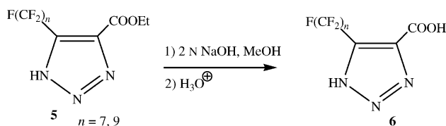
Scheme 9. Ester saponification.
