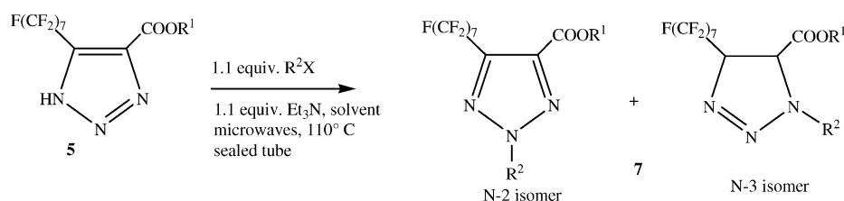
Scheme 10. Triazole alkylation.
