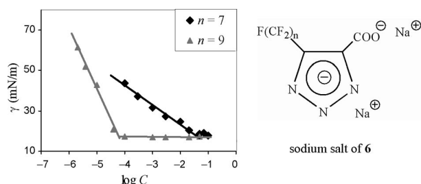
Figure 4. Surface activities of salt derivatives of 6 .
