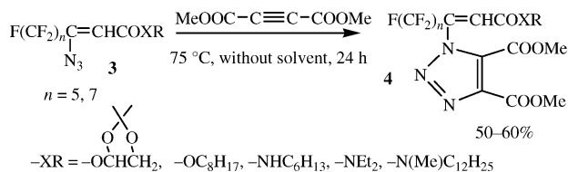
Scheme 3. 1,3-Dipolar cycloadditions with alkynes.
