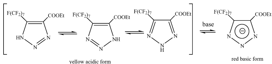
Scheme 8. Triazole deprotonation.
