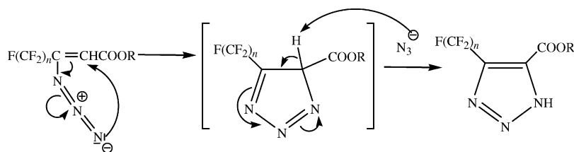
Scheme 6. First hypothesis for the mechanism of formation of triazole.
