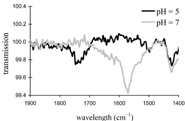
Figure 2. Changes in the IR spectrum of 6 ( n = 7 ) with the pH in aqueous solution.
