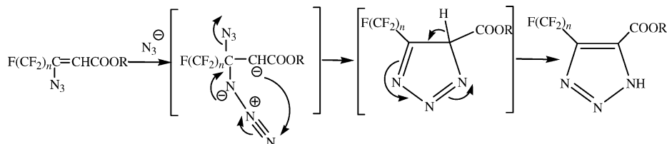
Scheme 7. Hypothesis for the mechanism of the triazole formation.
