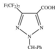
Figure 3. N-2 isomer of the acid derivative of 7c .
